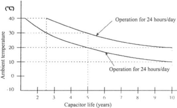
Fig.1.2. Capacitor life-time expectation depending on the ambient temperature in a low-power industrial diode-bridge VSI (reprinted from [41], pp. A-19, Appendix 5)
