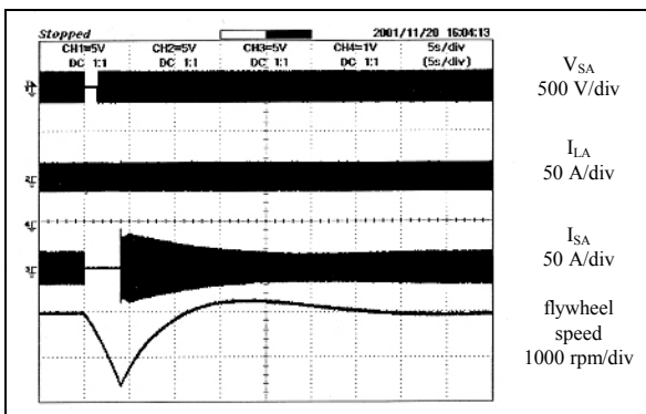
Fig. 11. Short interruption of the source supply
