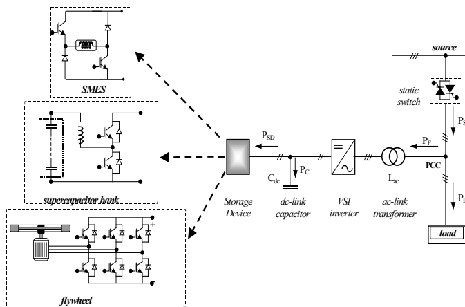
Fig. 1. Schematic drawing of the PCS structure
