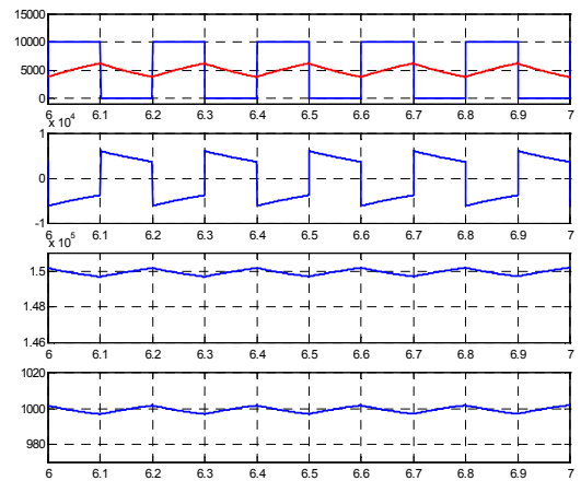
Fig. 5. Response of the PCS to a pulsating load. From the top to bottom: a) source and load instantaneous power P_S , P_L ; b) Storage device power P_{SD} ; c) Storage device energy E_{SD} ; d) dc-link capacitor energy E_C .
