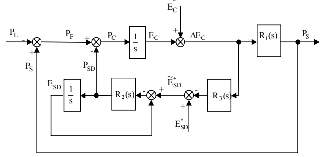
Fig. 3. Block diagram showing the relationship between P_L and P_S
