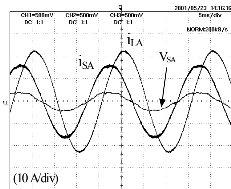
Fig. 9. Compensation of load reactive power
