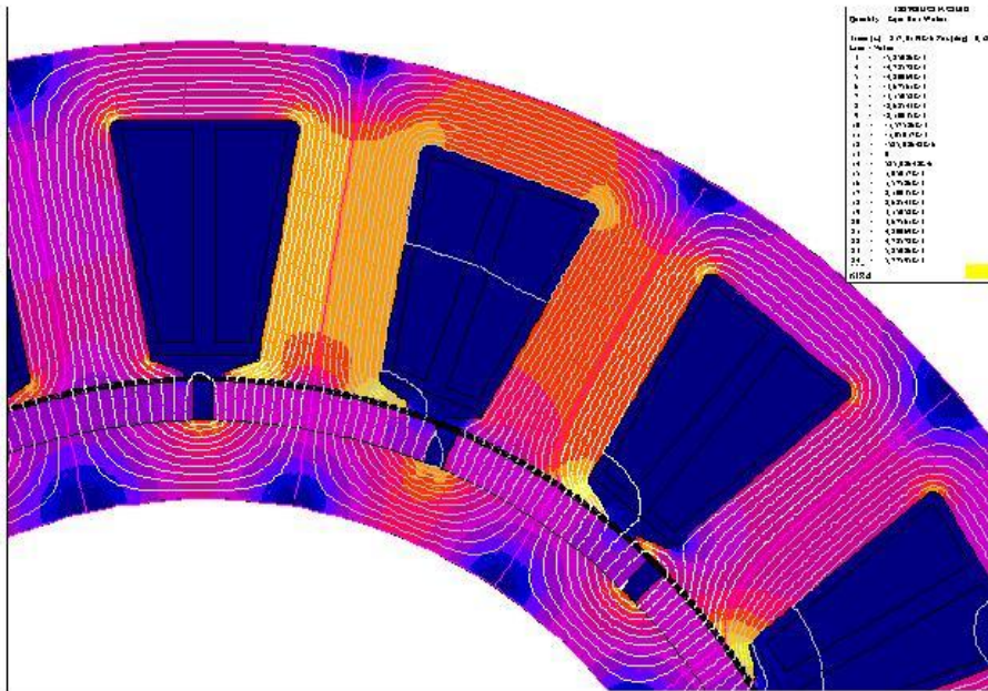
FEM analysis of an inner-rotor, surface-mounted PM brushless motor.
