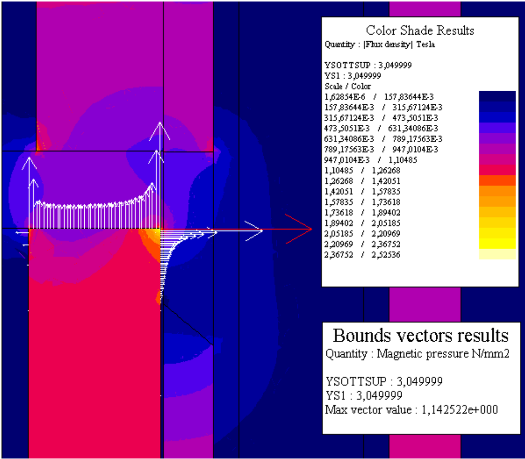
FEM analysis of an electromagnet
