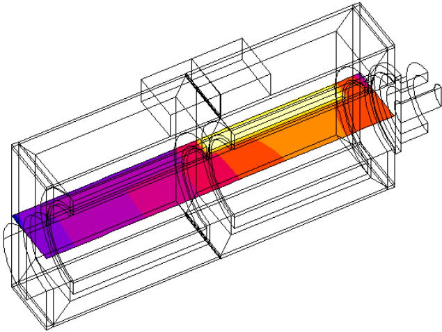
3D Thermal analysis of an electromagnet.
