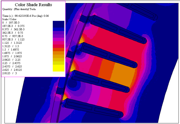
FEM analysis of outer-rotor, surface-mounted PM brushless motors.
