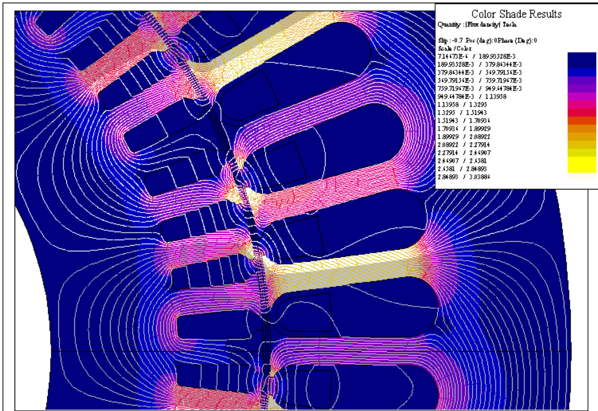
FEM analysis of a three-phase squirrel cage induction motor.
