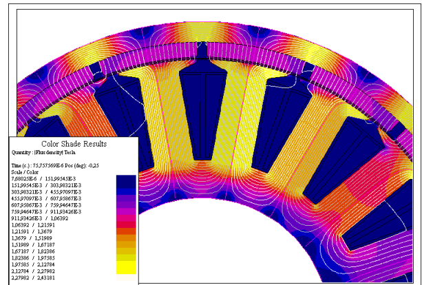
FEM analysis of outer-rotor, surface-mounted PM brushless motors.
