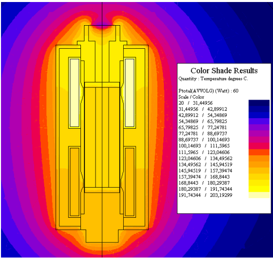
3D Thermal analysis of an electromagnet.
